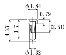
JS0020-GG-856 (J-856contact, Low force, Six fingers) Make to Order
