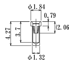
JS0020-GG-634 (J-634contact, High force)
